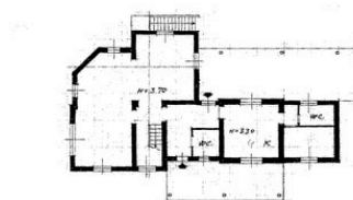
PIANO TERRA
