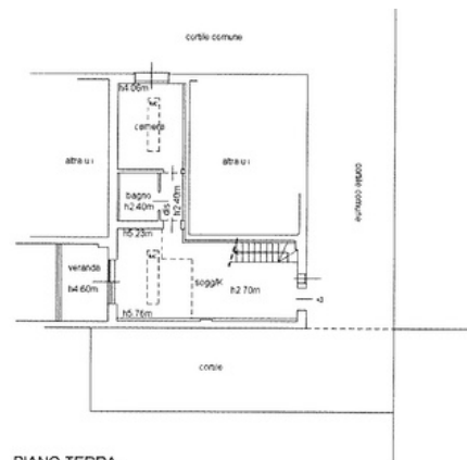
PIANO TERRA
