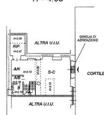
PIANO TERRENO H = 4.05
