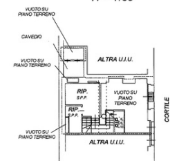
PIANO SOPPALCO H = 1.85
